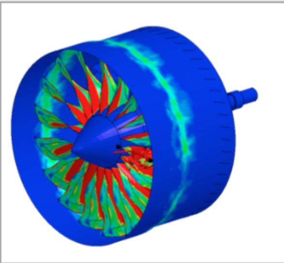
Figure IV.3 Engine damage 1.7 milliseconds following impact. The drone is mostly ingested, and high levels of stress are exerted on the engine blades.
